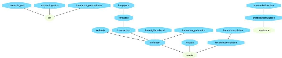
Figure 4: Object classes in the 'kstMatrix' package
