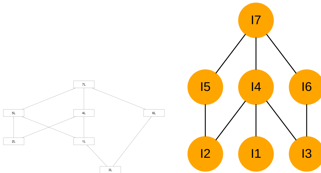
Figure 11: Implications determined by ‘DAKS’ compared to the true relation
