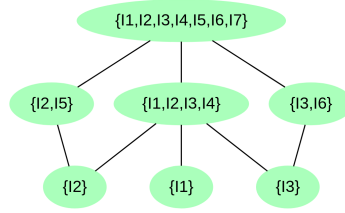
Figure 5: Plotting a basis with 'kstMatrix'
