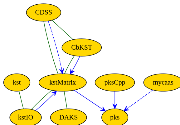
Figure 1: Network of R packages for knowledge space theory
