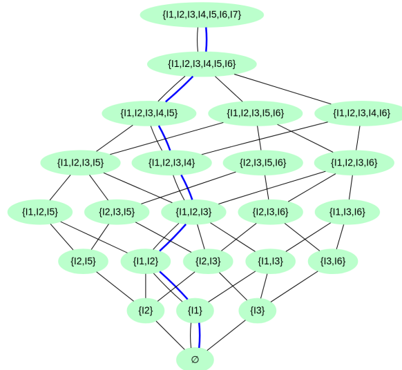
Figure 8: Learning path within a knowledge structure
